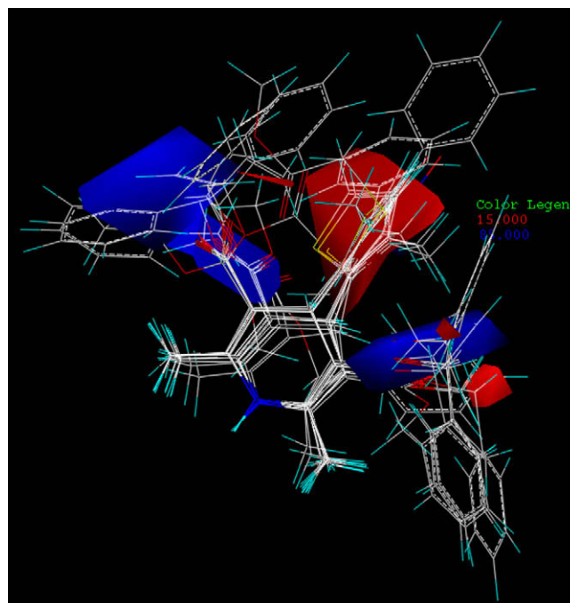
Figure 4. Contour maps of CoMFA electrostatic regions are shown around the studied compounds. Blue regions are favourable for more positively charged groups; red regions are favourable for less positively charged groups.
